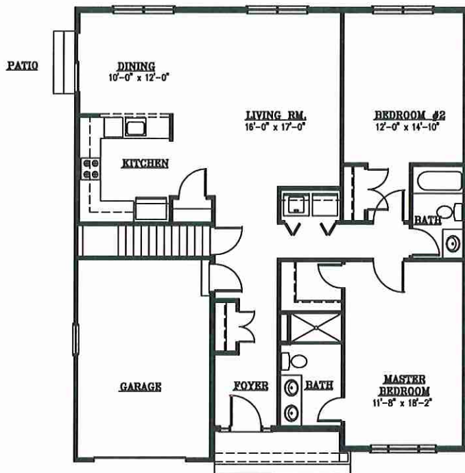
FIRST FLOOR PLAN FIRST FLOOR = 1382 SF
