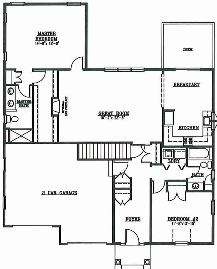
FIRST FLOOR PLAN FIRST FLOOR = 1618 SF
