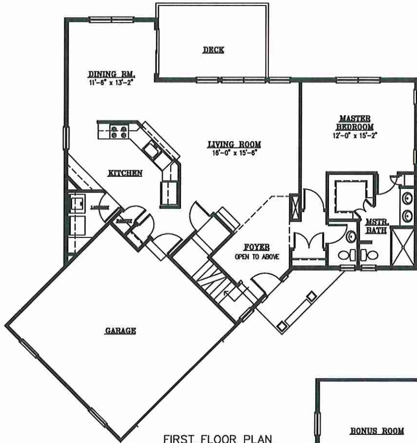
FIRST FLOOR PLAN FIRST FLOOR = 1300 SF SECOND FLOOR = 860 SF TOTAL = 2160 SF BONUS ROOM = (170) SF
